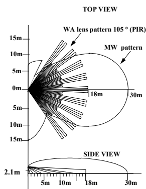
FIG. 5 - WA PIR + MW DETECTION PATTERN
