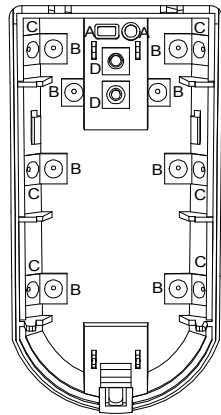
FIG. 2 - KNOCKOUT HOLES
