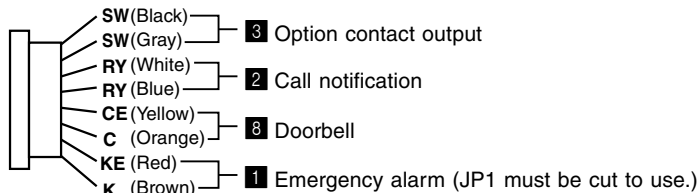
Option connector
